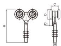
四轮轴承挂轮 (304, stainless steel) Hanging Door Roller (4 Rollers, Forge Centre Plate)
