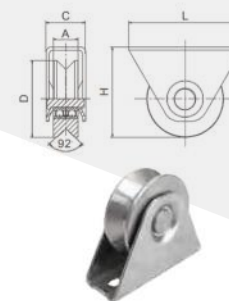
梯形V槽双轴承滑轮 (304, stainless steel) Sliding Gate Wheel with Exterior Bracket(Double Bearings, V groove)
