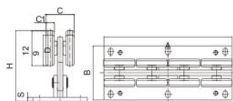
大八轮 8 Large Wheels
