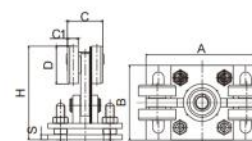
70x70升降五轮 5 Wheels, for 70X70 Track
