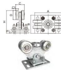
80x80升降五轮 5 Wheels, for 80X80 Track
