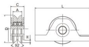
叠片Y槽双轴承滑轮 (304, stainless steel)
