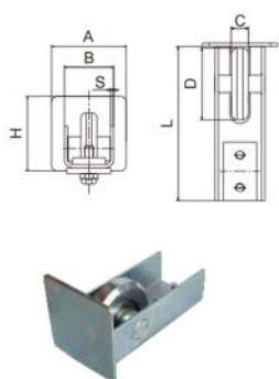
80x80五轮导轮 Guide Wheel
