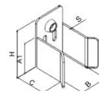
不带底板门兜 Gate Catcher (without Base Plate)
