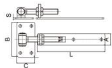
木门铰链 Wooden Gate Hinge
