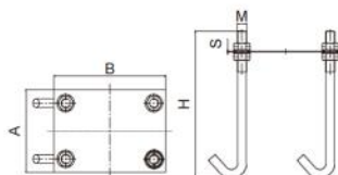
小五轮底座 Adjustable Fixing Plate with Hook Bolt
