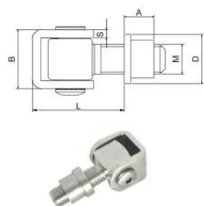
方头螺帽铰链 (304, stainless steel) Adjustable Gate Hinge with Nut
