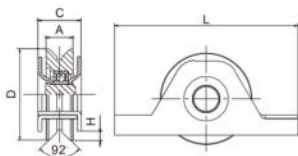
叠片Y槽单轴承滑轮 (304, stainless steel)
