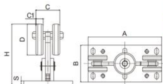
大五轮 5 Large Wheels
