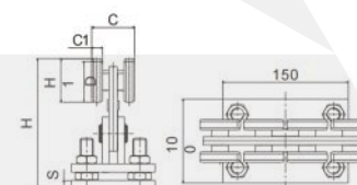
升降中八轮 Adjustable 8 Medium Wheels
