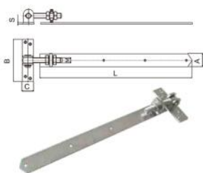
长板铰链 (304, stainless steel) Wooden Gate Hinge
