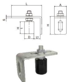
可调单轮L型框架 Guide Bracket with Nylon Roller
