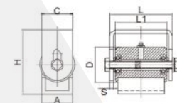
可调虎头铰链 Standard Duty Round Mount Hinge
