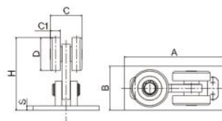
不升降三轮 3 Wheels for 80x80 Track
