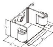
双轮门兜 Gate Catcher (with 2 Nylon Rollers)
