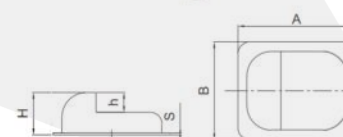
拖鞋门吸 (304, stainless steel) Gate Stopper with Base Plate for Two Leaf Gate
