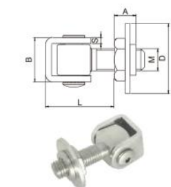
方头圆片铰链 (304, stainless steel) Adjustable Gate Hinge with Round Plate
