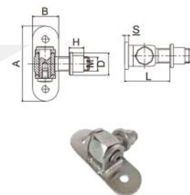
带焊接板欧式螺帽铰链 (304, stainless steel) Adjustable Gate Hinge with Square Plate
