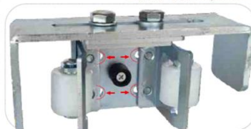
2. 门兜可调 AdjustableBracket
