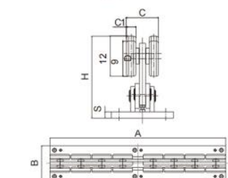
大十六轮 16 Large Wheels
