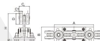
升降悬轮 (十轮) 10 Wheels for 80X80 Track
