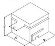
澳洲塑料方块 Plastic Block
