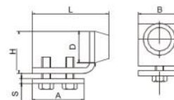
挂轮门吸 Stopper for Track
