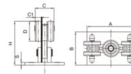
东欧升降五轮 (精简款) (80x80) (304, stainless steel) Adjustable Cantilever Gate Carriage (5 Wheels, for 80X80 Track)
