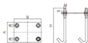
小八轮底座 Adjustable Fixing Plate with Hook Bolt
