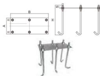
大八轮底座 Fixing Plate with Hook Bolt
