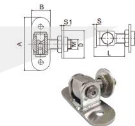
带焊接板欧式圆片铰链 (304, stainless steel) Adjustable Gate Hinge with Square Plate
