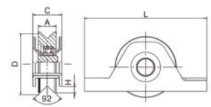
叠片V槽单轴承滑轮 (304, stainless steel)
