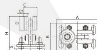
升降三轮 3 Wheels, for 80X80 Track
