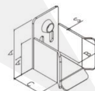
70x70五轮门兜 Gate Catcher
