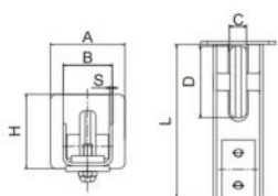
60x60五轮导轮 Guide Wheel
