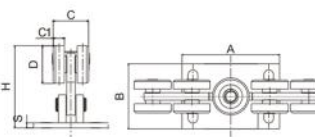
不升降九轮 9 Wheels, for 80X80 Track
