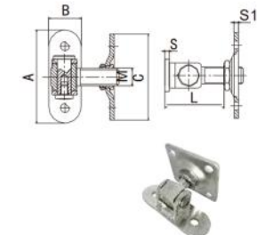
带焊接板欧式方片铰链 (304, stainless steel) Adjustable Gate Hinge with Square Plate
