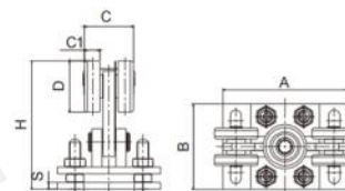
60x60升降五轮 5 Wheels, for 60X60 Track
