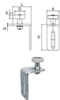
扁轮框架 Guide Bracket with Nylon Roller
