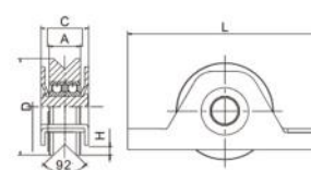
叠片V槽双轴承滑轮 (304, stainless steel)
