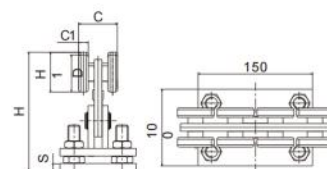
升降小八轮 Adjustable 8 Small Wheels
