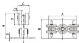
东欧五轮 (60x60) (304, stainless steel) Cantilever Gate Carriage (5 Wheels, for 60X60 Track)
