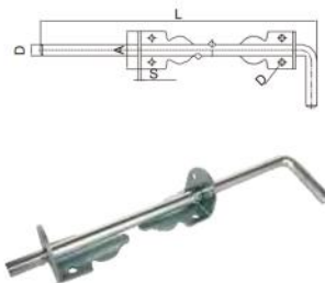
长L插销 Gate Latch
