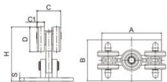
60x60五轮 5 Wheels, for 60X60 Track
