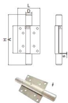
不锈钢合页弹簧铰链 spring hinge of 304ss
