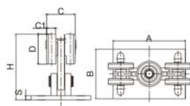
70x70不升降五轮 5 Wheels, for 70X70 Track
