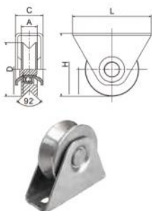
梯形V槽单轴承滑轮 (304, stainless steel) Sliding Gate Wheel with Exterior Bracket(Single Bearing, V groove)
