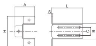
门兜托架 Bracket for Gate Catcher
