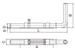
七字插销 Gate Latch
