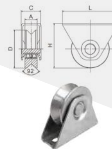
梯形V槽双轴承滑轮 (304, stainless steel) Sliding Gate Wheel with Exterior Bracket(Double Bearings, V groove)
