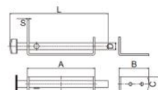
双L插销 Gate Latch
