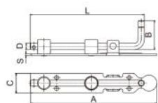
双柱插销 Gate Latch
