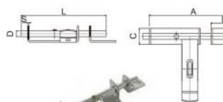
双T插销 Gate Latch
