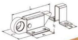
Q型插销 Gate Latch
