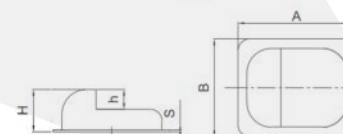
拖鞋门吸 (304, stainless steel) Gate Stopper with Base Plate for Two Leaf Gate
