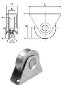
梯形V槽单轴承滑轮 (304, stainless steel) Sliding Gate Wheel with Exterior Bracket(Single Bearing, V groove)
