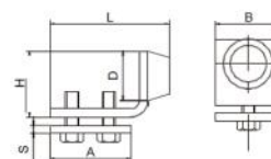
挂轮门吸 Stopper for Track
